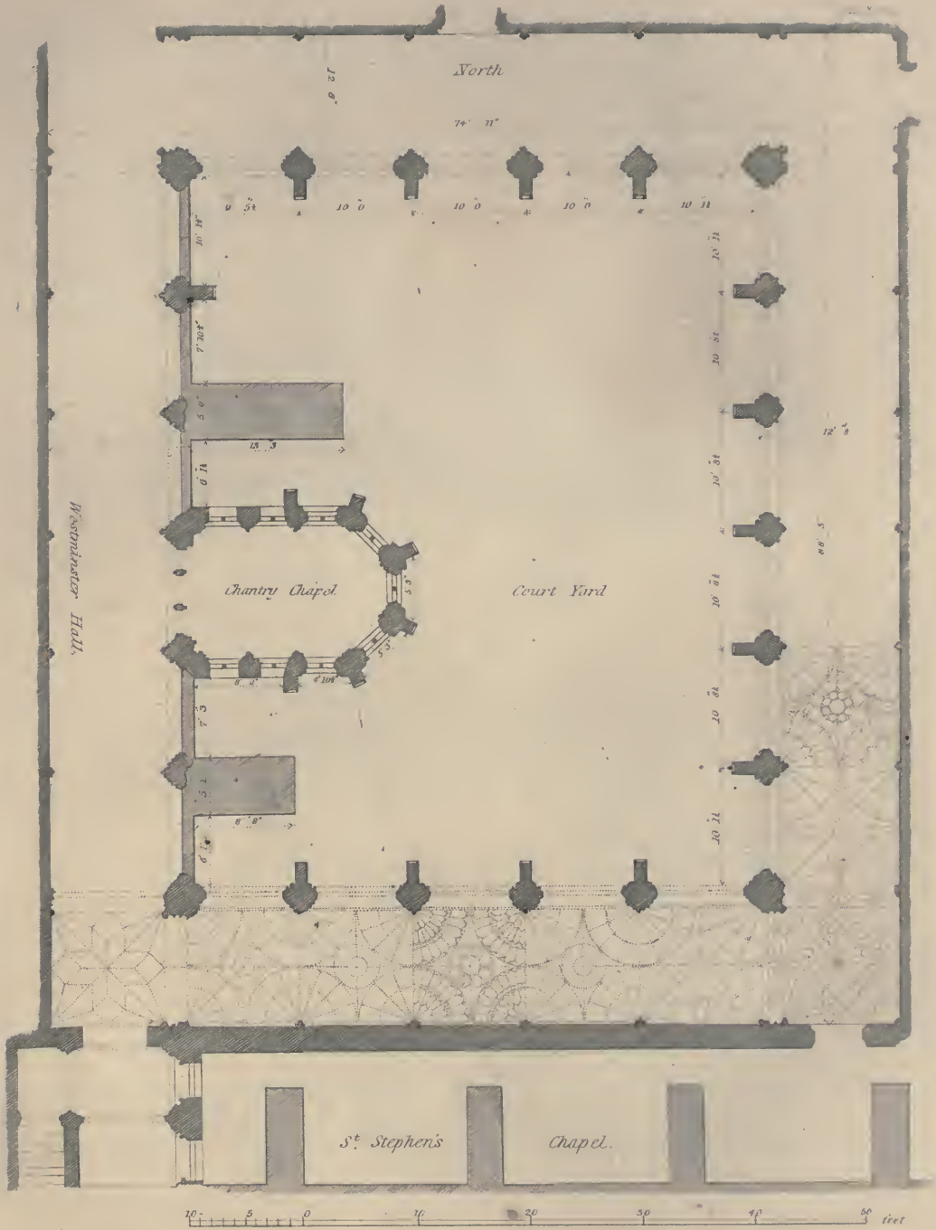
PLAN OF CLOISTERS ST. STEPHEN'S CHAPEL, WESTMINSTER.
